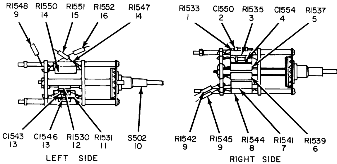
SWITCH ASSEMBLY A1502
