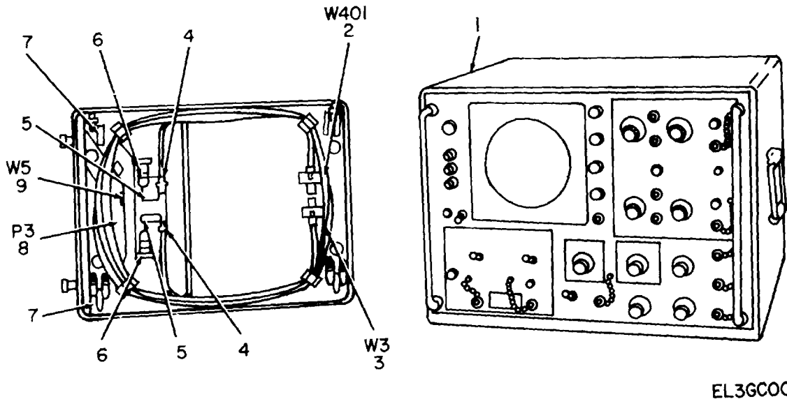
Figure 1. Oscilloscope AN/USM-140A.
