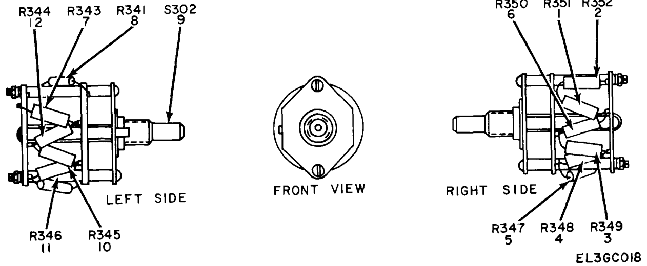
Figure 14. Oscilloscope Assembly US-IZI/USM-14UA, Switch Assembly eye.
