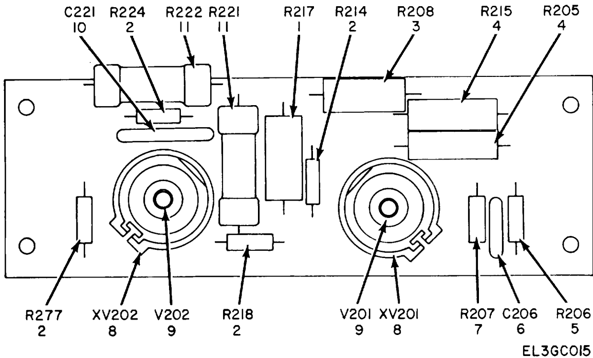
Figure 11. Oscilloscope Assembly OS-121/USM-140A, Etched Circuit Board Assembly A201.
