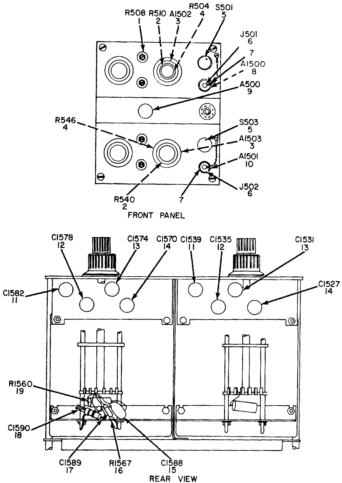
Figure 20. Preamplifier, Dual Trace MX-2930A/USHI (Sheet 1 of 2).
