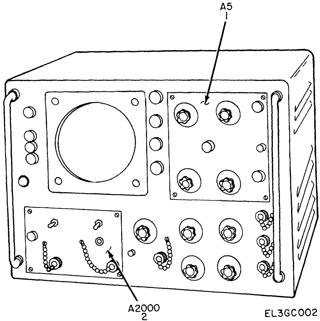
Figure 2. Oscilloscope Assembly OS-121/USM-140A, Location of Subassemblies.
