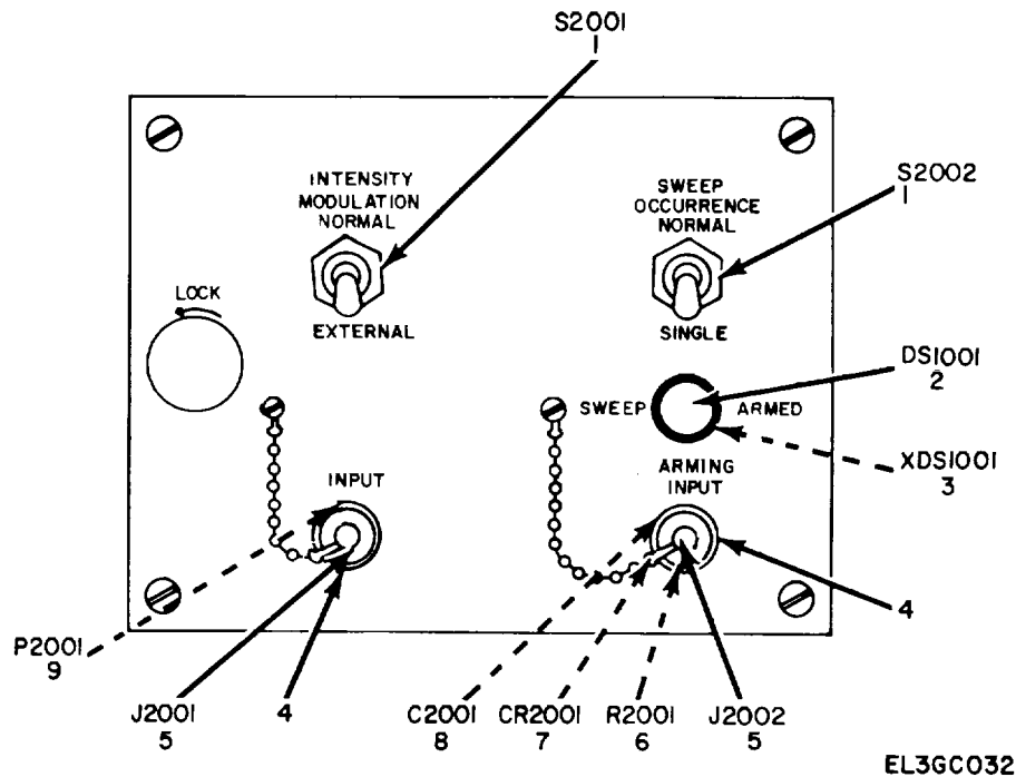
Figure 27. Auxiliary Plug-In MX-3078/USM.
