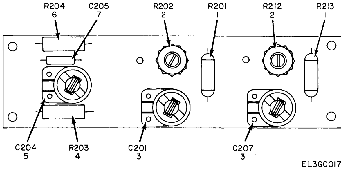
Figure 13. Oscilloscope Assembly OS-121/USM-140A, Etched Circuit Board Assembly A203.
