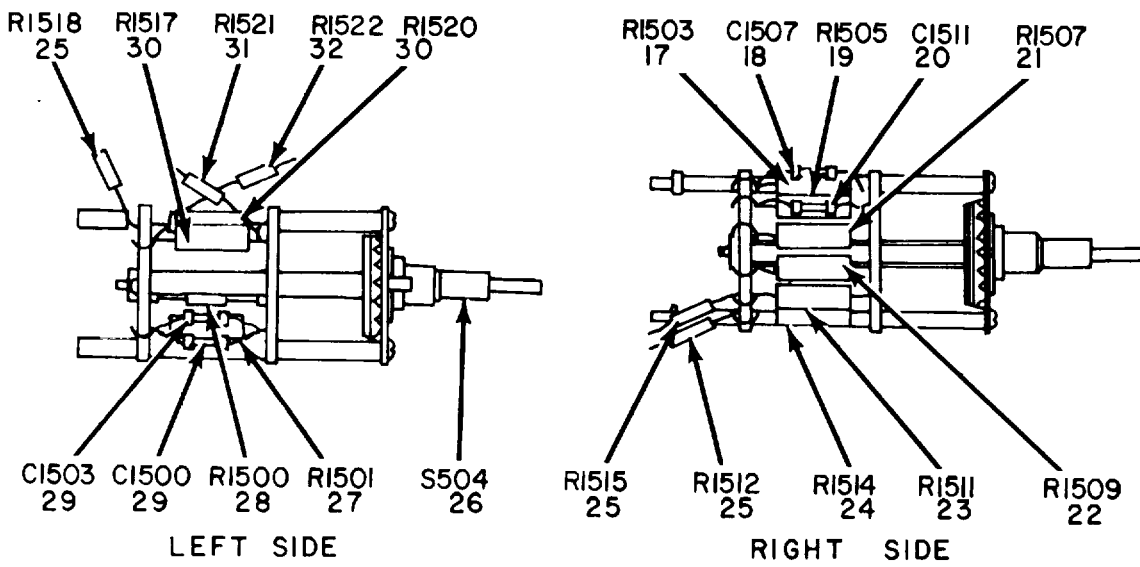
SWITCH ASSEMBLY A1503
