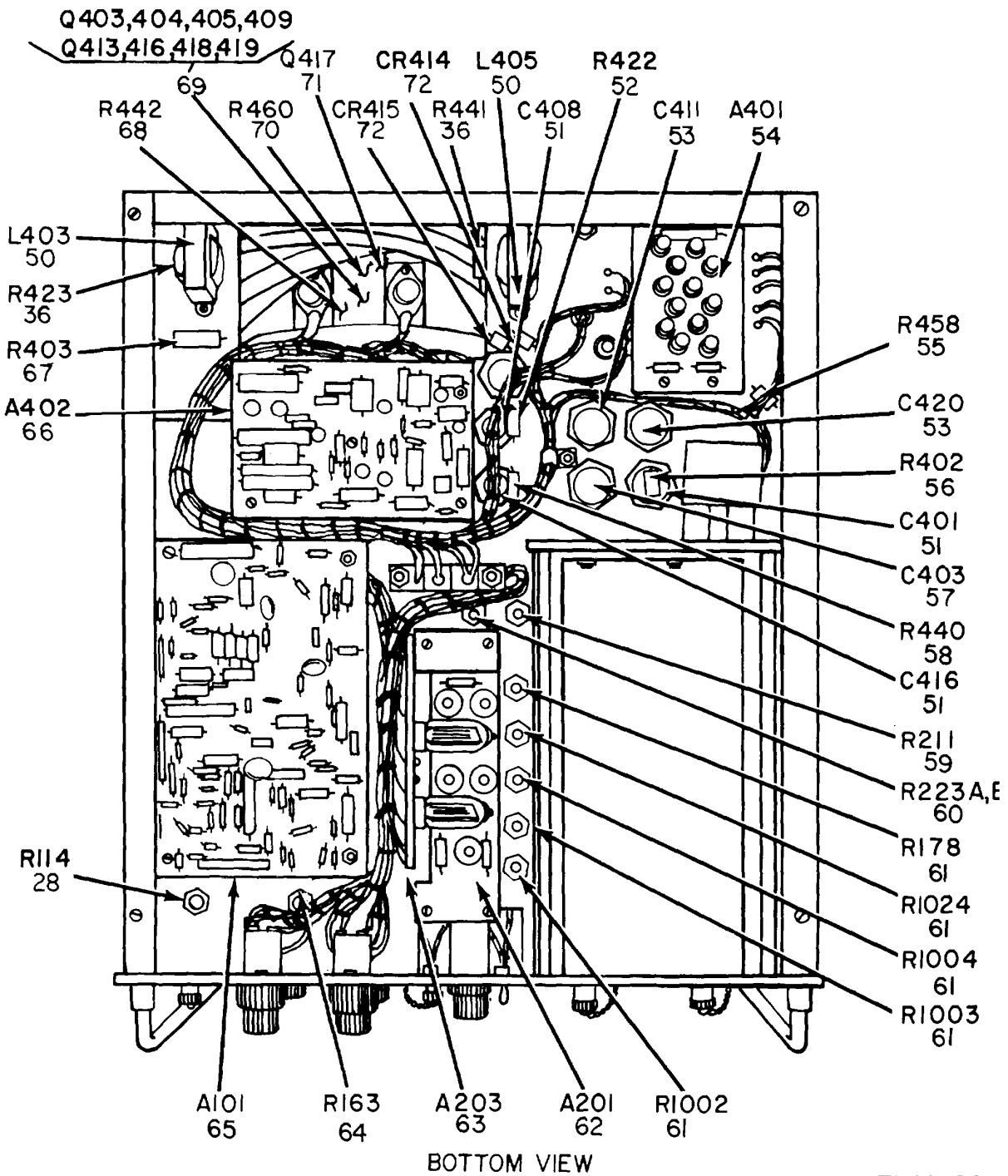
Figure 3. Oscilloscope Assembly OS-121/USM-140A (Sheet 3 of 5).
