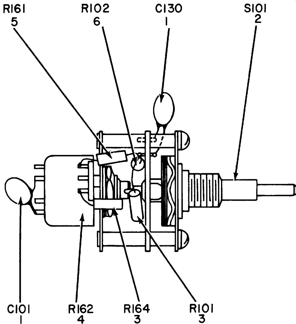
Figure 9. Oscilloscope Assembly OS-121/USM-140A, Switch Assembly A102.
