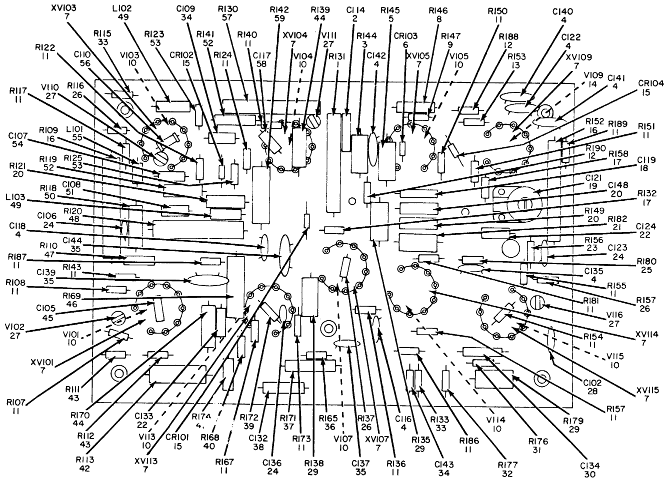
Figure 8. Oscilloscope Assembly OS-121/USM-140A, Etched Circuit Board Assembly A101. EL3GCO2
