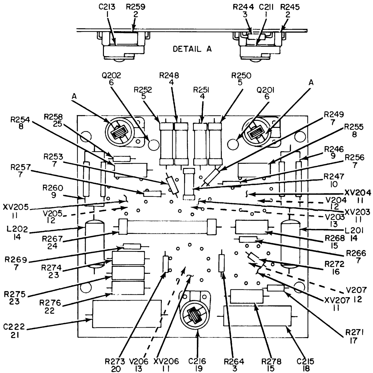
Figure 12. Oscilloscope Assembly OS-121/USM-140A, Etched Circuit Board Assembly A202.
