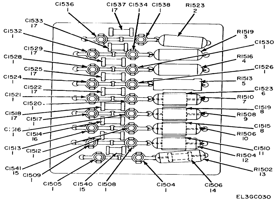
Figure 25. Preamplifier, Dual Trace MX-2930A/USM, Attenuator Assembly, Channel B A1501.
