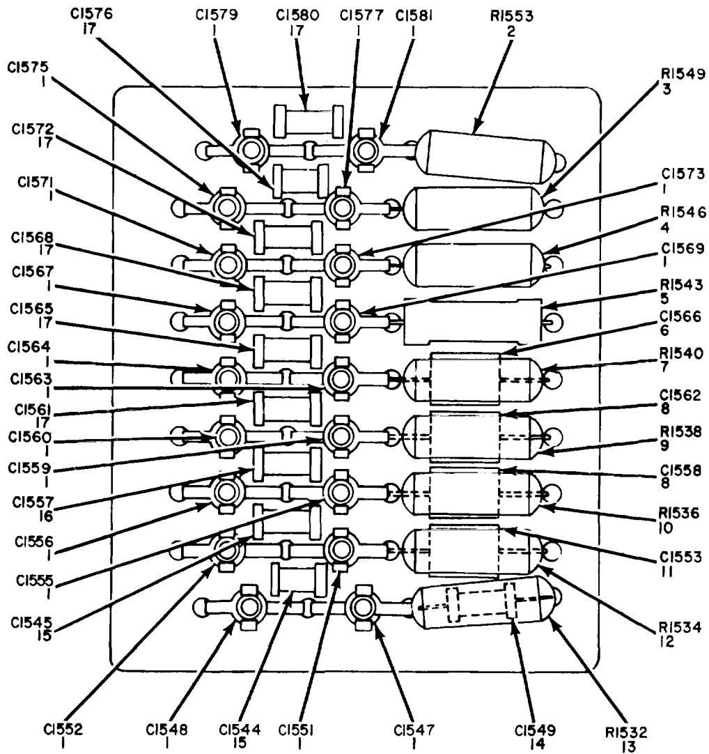
Figure 24. Preamplifier, Dual Trace MX-2930A/USM, Attenuator Assembly, Channel A A1500.
