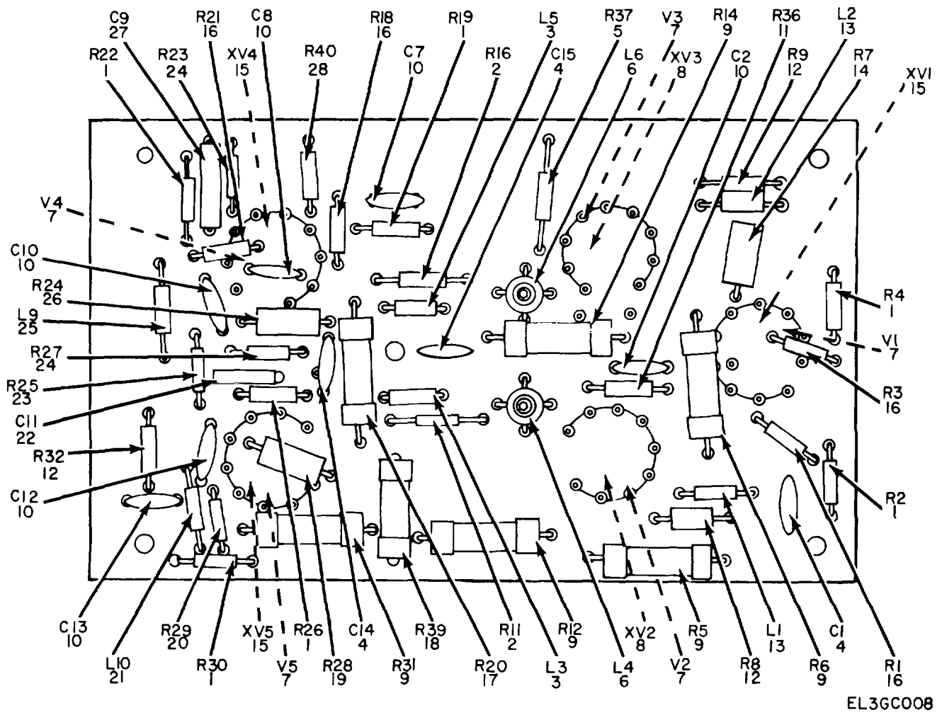
Figure 4. Oscilloscope Assembly OS-121/USM-140A, Etched Circuit Board A1.
