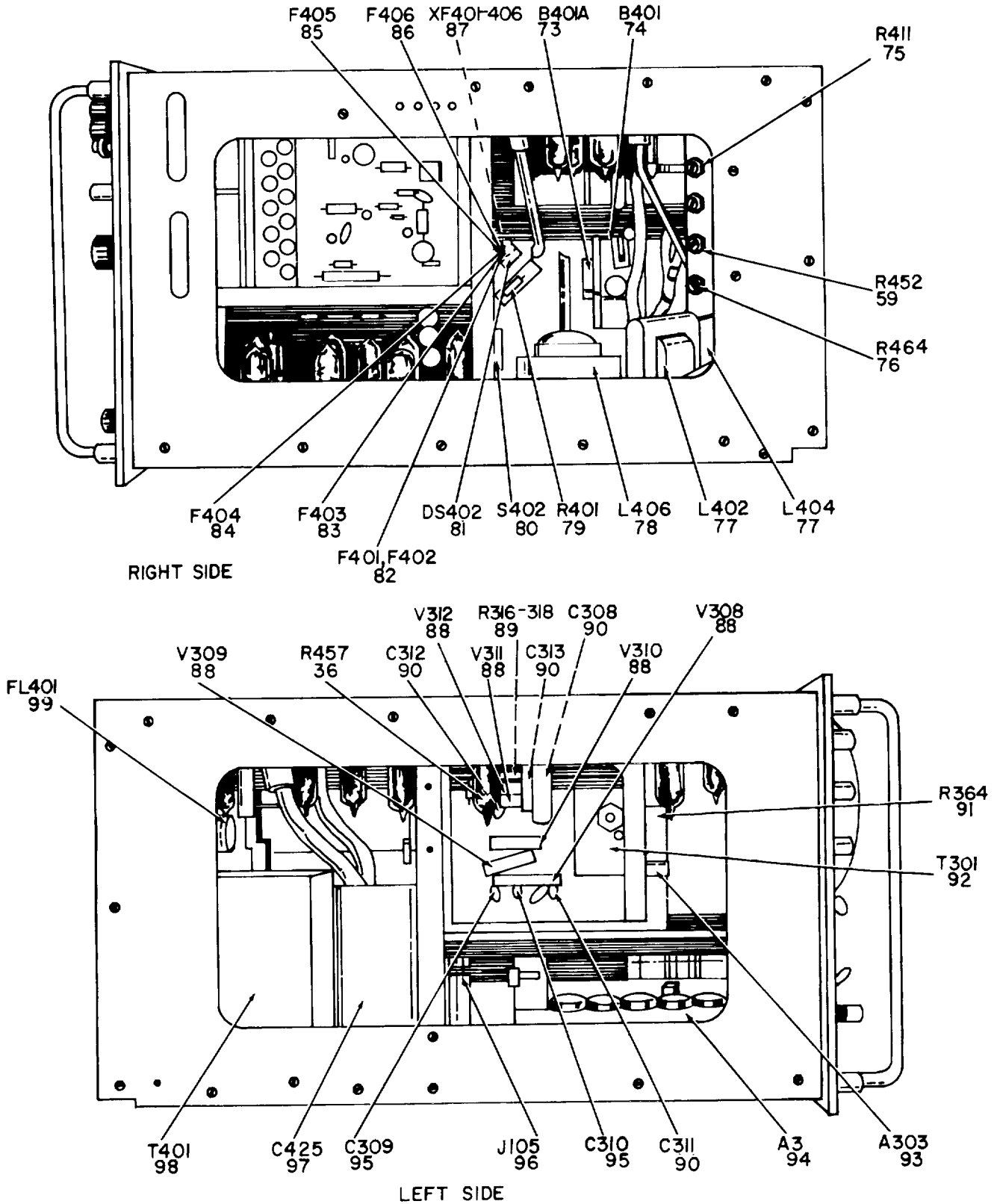
Figure 3. Oscilloscope Assembly OS-121/USM-140A (Sheet 4 of 5).
