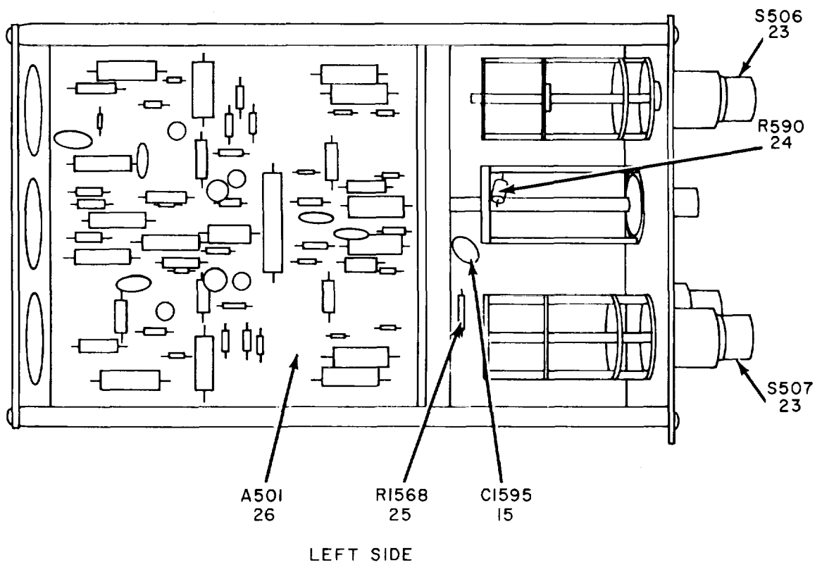
Figure 20. Preamplifier, Dual Trace MX-2930A/USM (Sheet 2 of 2).
