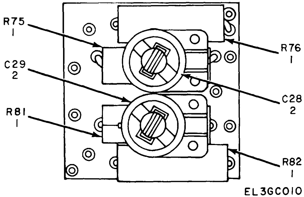
Figure 6. Oscilloscope Assembly OS-121/USM-140A, Etched Circuit Board A3
